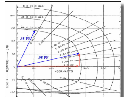
Generator Capability Curves
